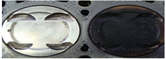
Piston crown with heavy deposit build-up. Piston crown after service.
